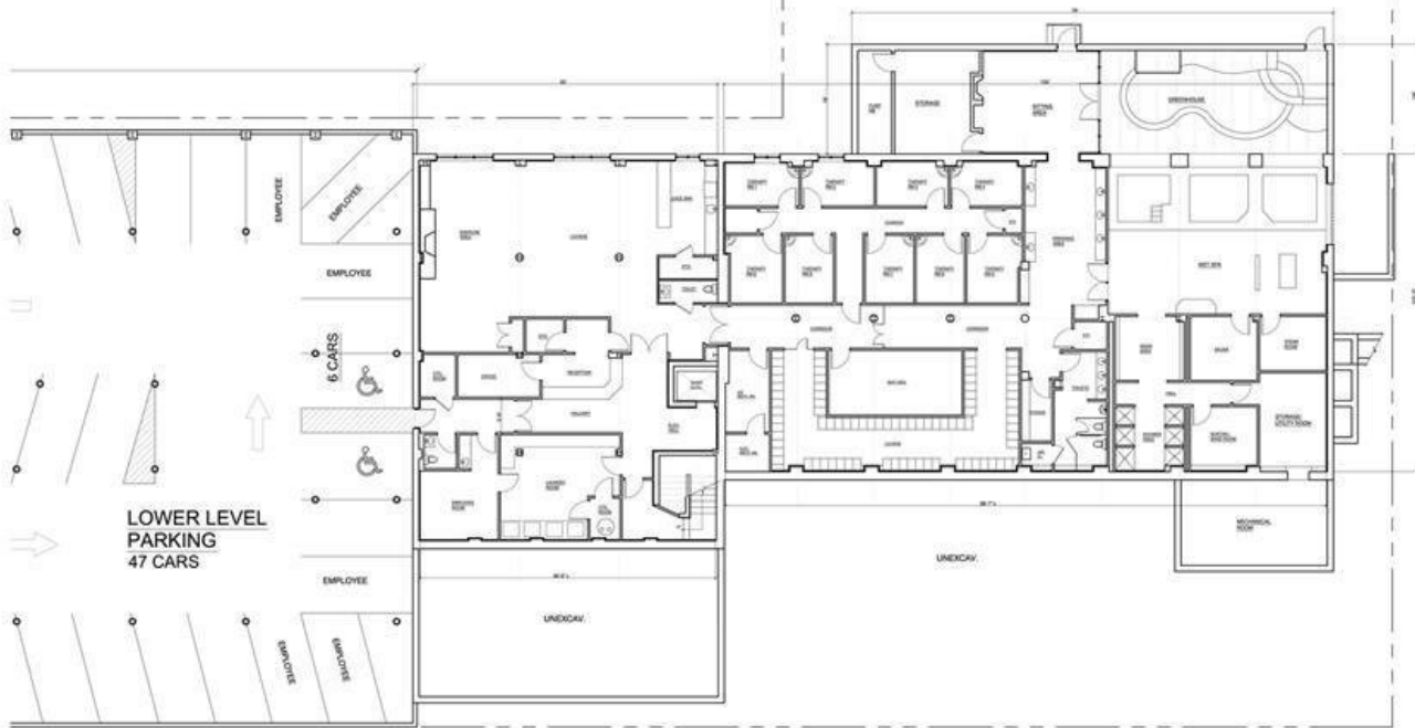
BASEMENT PLAN SCALE: 1/8" (EXISTING MEN'S SPA) SPA FLOOR AREA: 10,470 SF
